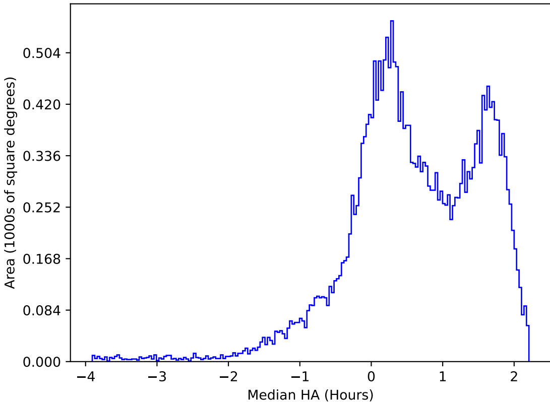
ddf_acor_sf15_ls30_lsr10_v3.4_10yrs All sky g band: Median HA
