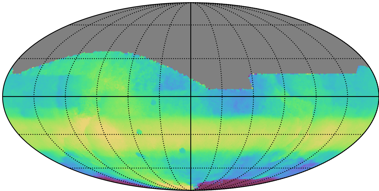
ddf_acor_sf15_lsf30_lsr10_v3.4_10yrs All sky all bands: Median HA
