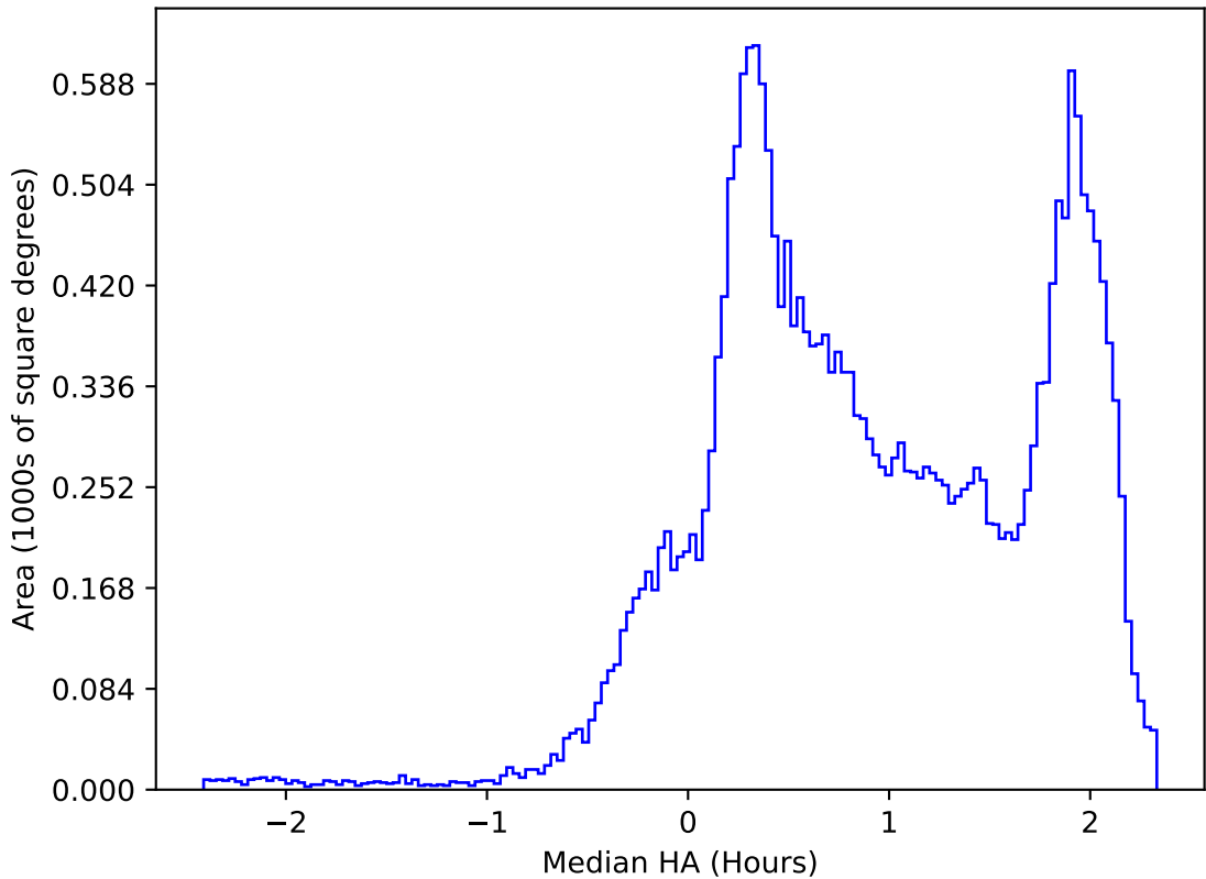
ddf_acor_sf15_lsf30_lsr10_v3.4_10yrs All sky all bands: Median HA
