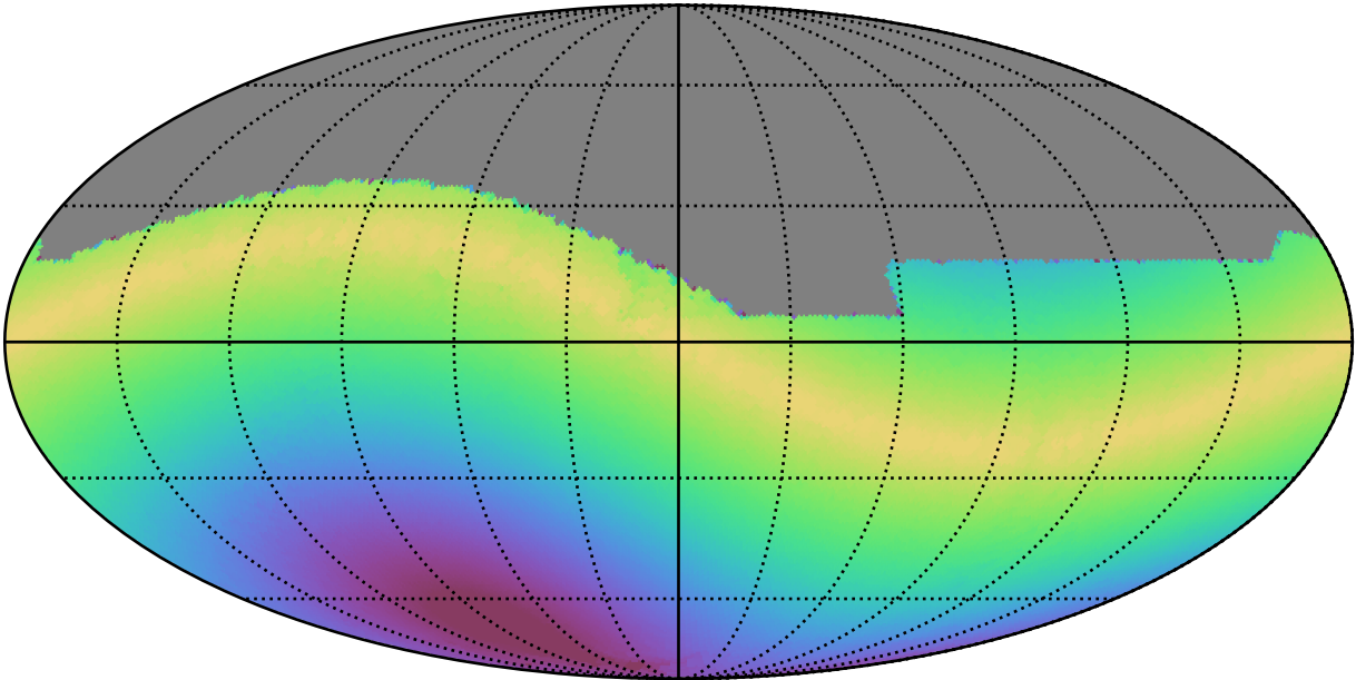
ddf_acor_sf15_lsf30_lsr10_v3.4_10yrs All sky r band: Max solarElong
