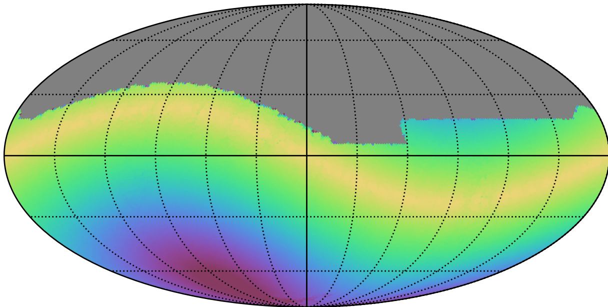
ddf_acor_sf15_lsf30_lsr10_v3.4_10yrs All sky i band: Max solarElong
