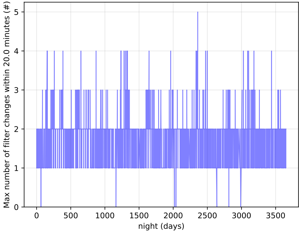
ddf_acor_sf15_Isf30_Isr10_v3.4_10yrs Per Night: Max number of filter changes within 20.0 minutes
