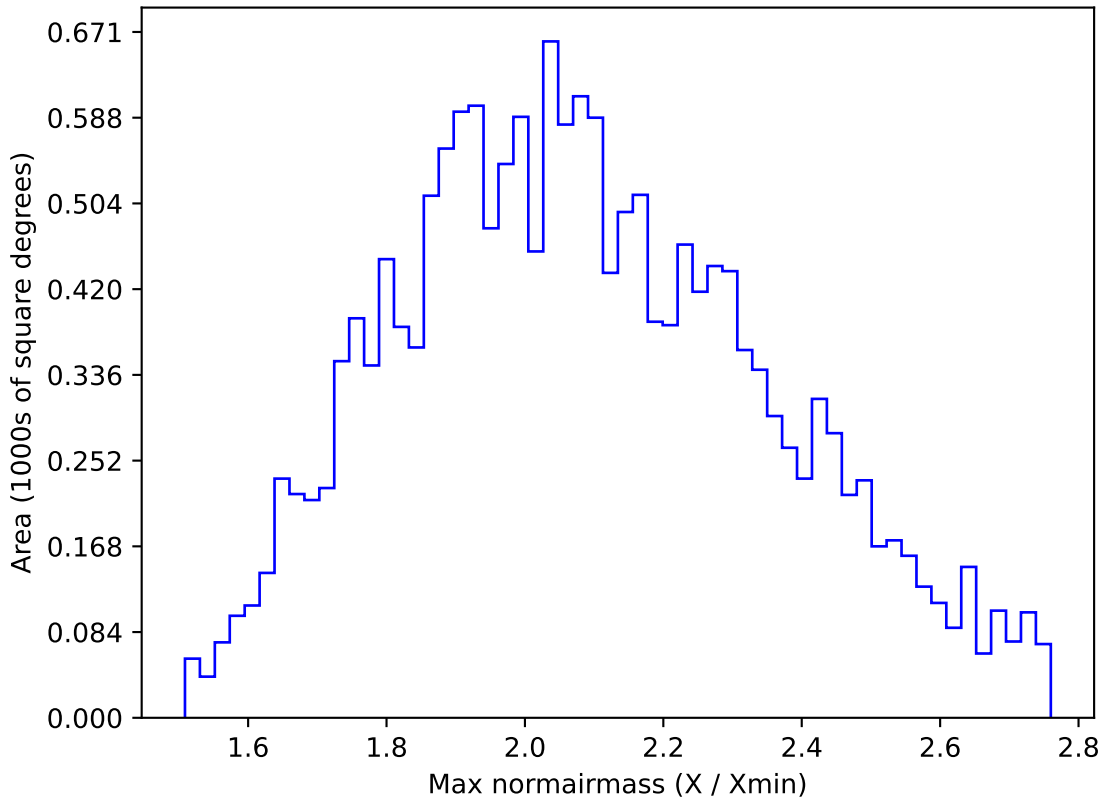
ddf_acor_sf15_lsf30_lsr10_v3.4_10yrs WFD y band: Max normairmass
