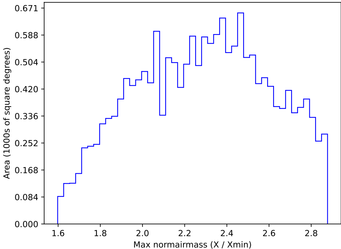
ddf_acor_sf15_lsf30_lsr10_v3.4_10yrs WFD i band: Max normairmass
