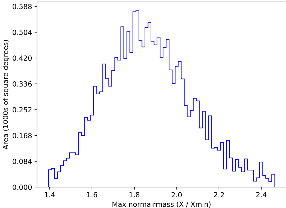
ddf_acor_sf15_lsf30_lsr10_v3.4_10yrs WFD g band: Max normairmass
