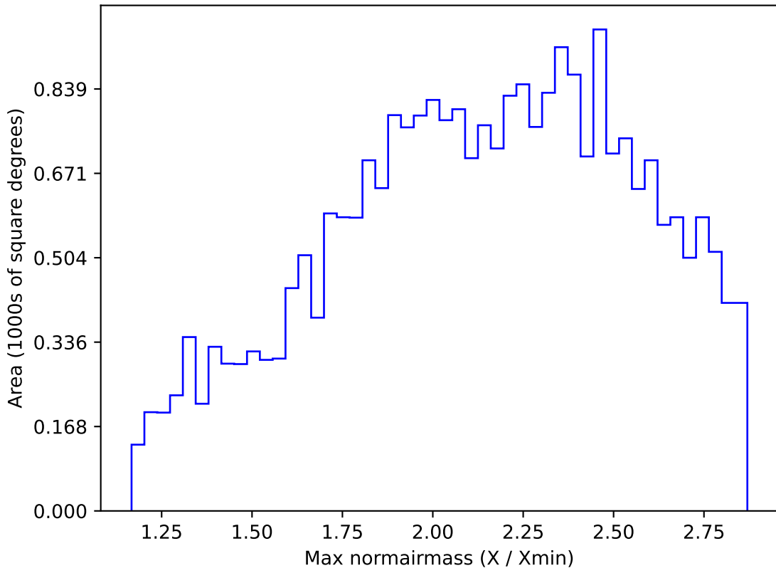
ddf_acor_sf15_lsf30_lsr10_v3.4_10yrs All sky i band: Max normairmass
