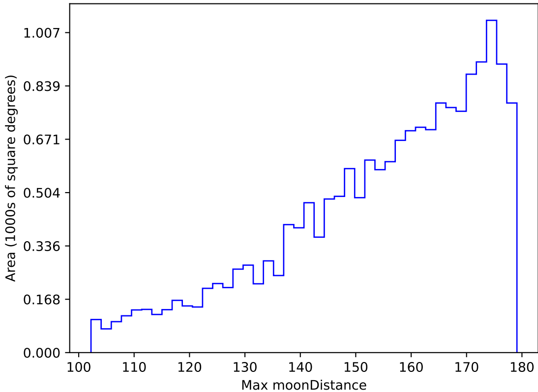
ddf_acor_sf15_lsf30_lsr10_v3.4_10yrs WFD u band: Max moonDistance
