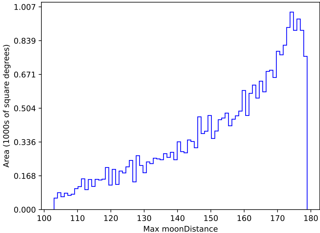
ddf_acor_sf15_lsf30_lsr10_v3.4_10yrs All sky g band: Max moonDistance
