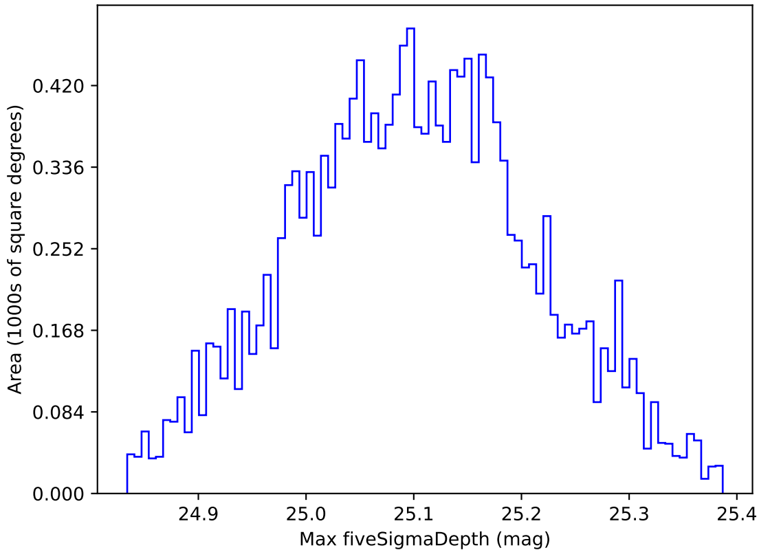
ddf_acor_sf15_lsf30_lsr10_v3.4_10yrs WFD all bands: Max fiveSigmaDepth
