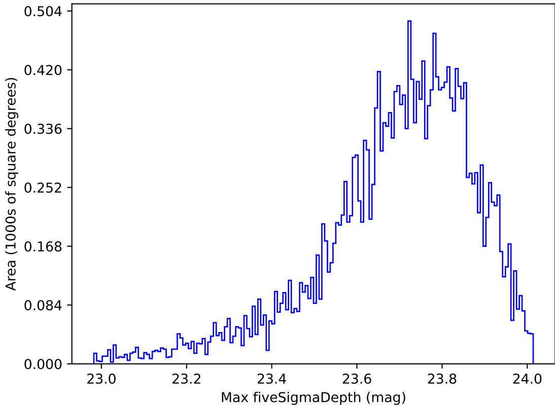
ddf_acor_sf15_ls30_lsr10_v3.4_10yrs All sky u band: Max fiveSigmaDepth
