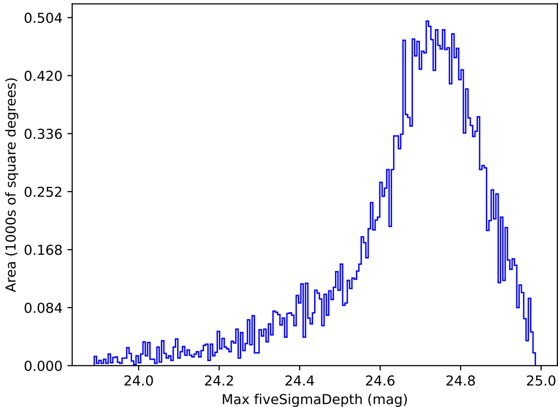
ddf_acor_sf15_lsf30_lsr10_v3.4_10yrs All sky r band: Max fiveSigmaDepth
