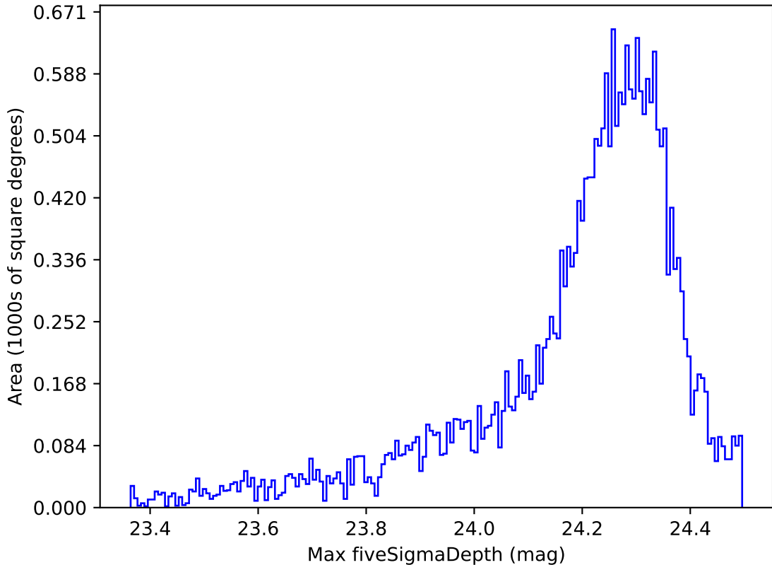
ddf_acor_sf15_lsf30_lsr10_v3.4_10yrs All sky i band: Max fiveSigmaDepth
