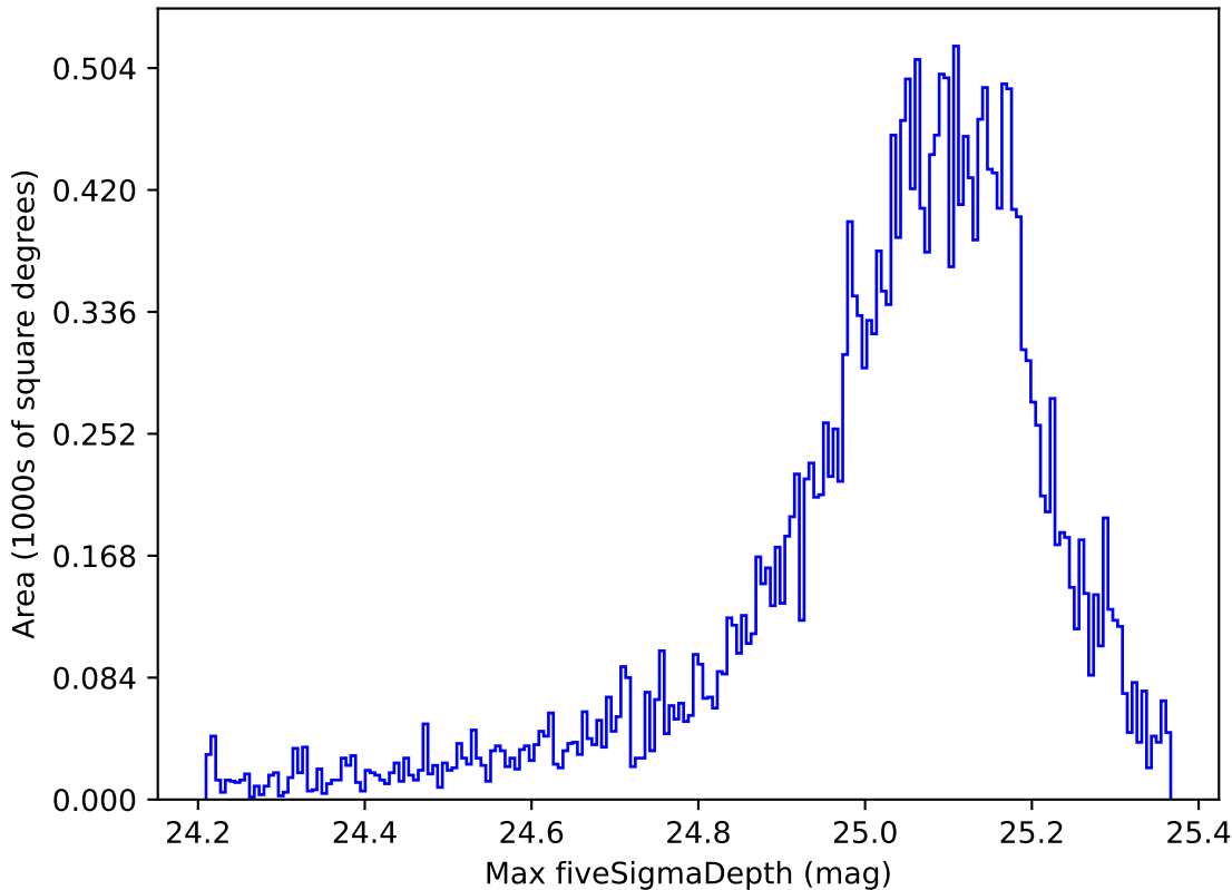
ddf_acor_sf15_ls30_lsr10_v3.4_10yrs All sky g band: Max fiveSigmaDepth
