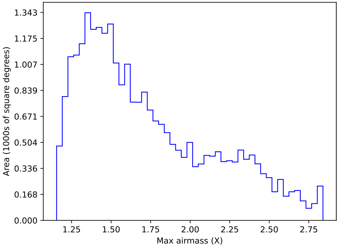
ddf_acor_sf15_lsf30_lsr10_v3.4_10yrs Yr 1 z band: Max airmass
