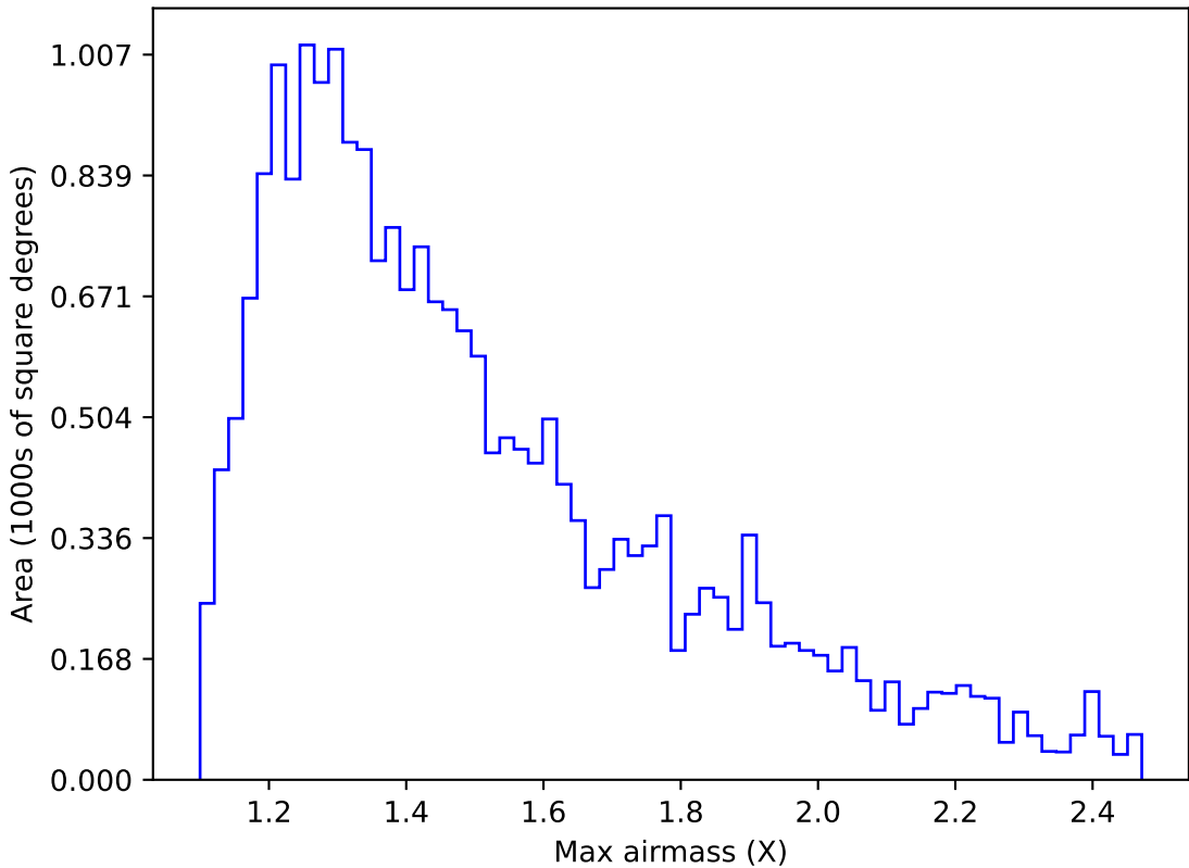
ddf_acor_sf15_lsf30_lsr10_v3.4_10yrs Yr 1 u band: Max airmass
