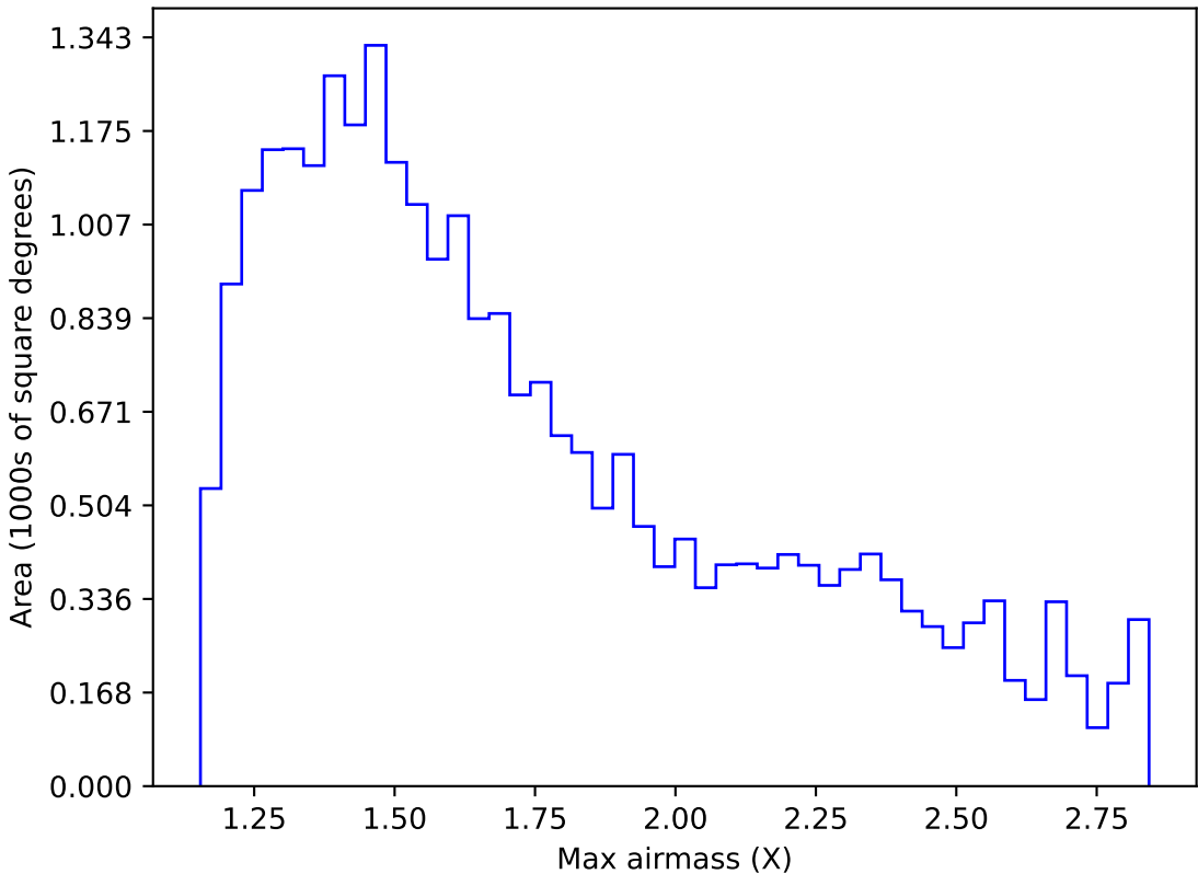
ddf_acor_sf15_lsf30_lsr10_v3.4_10yrs Yr 1 i band: Max airmass
