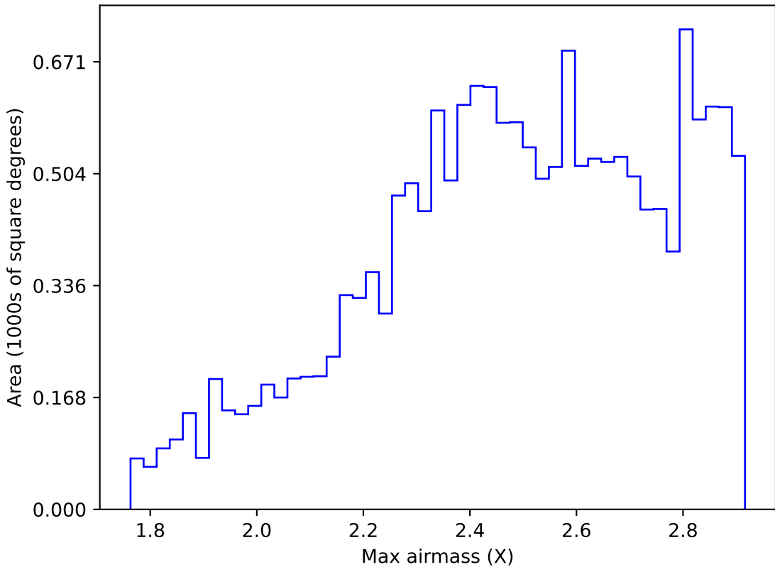
ddf_acor_sf15_lsf30_lsr10_v3.4_10yrs WFD z band: Max airmass
