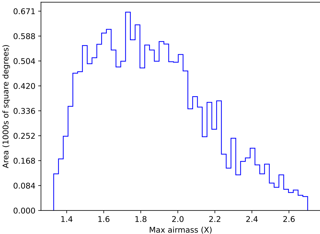
ddf_acor_sf15_ls30_lsr10_v3.4_10yrs WFD u band: Max airmass
