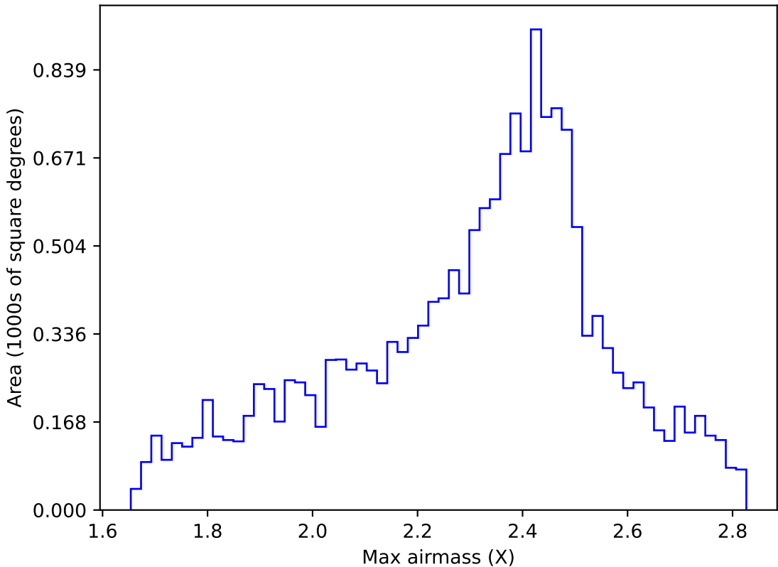
ddf_acor_sf15_lsf30_lsr10_v3.4_10yrs WFD r band: Max airmass
