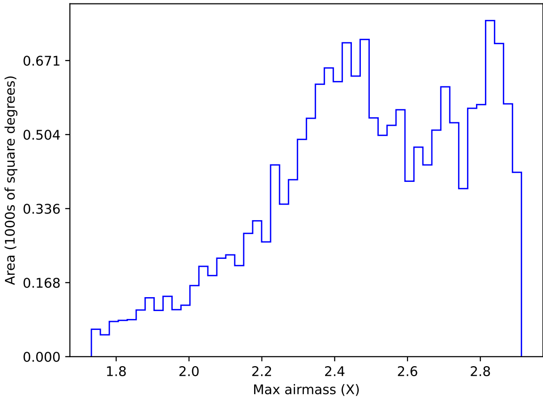
ddf_acor_sf15_lsf30_lsr10_v3.4_10yrs WFD i band: Max airmass
