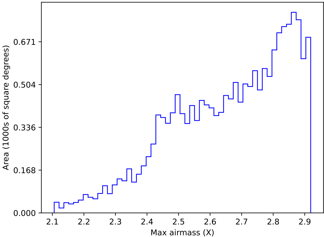
ddf_acor_sf15_lsf30_lsr10_v3.4_10yrs WFD all bands: Max airmass
