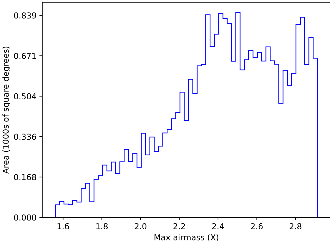
ddf_acor_sf15_lsf30_lsr10_v3.4_10yrs All sky z band: Max airmass
