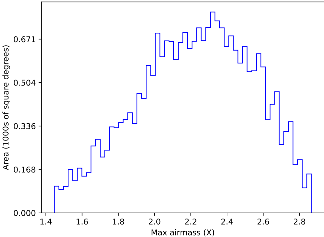
ddf_acor_sf15_lsf30_lsr10_v3.4_10yrs All sky y band: Max airmass
