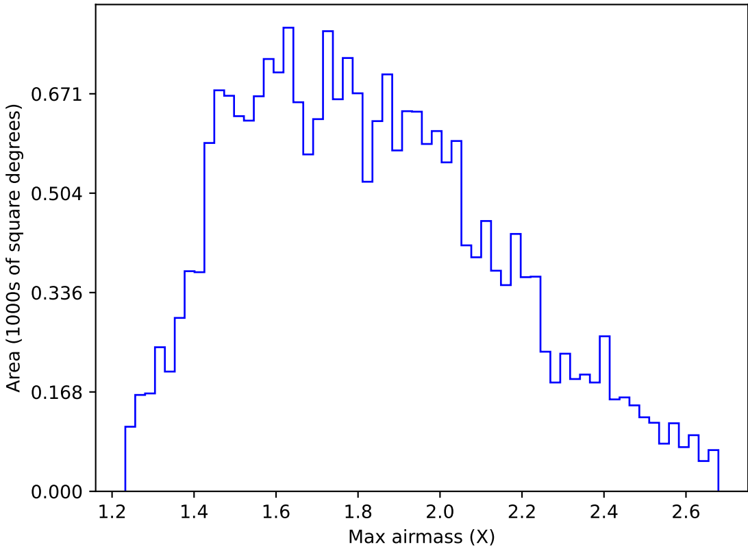
ddf_acor_sf15_lsf30_lsr10_v3.4_10yrs All sky u band: Max airmass
