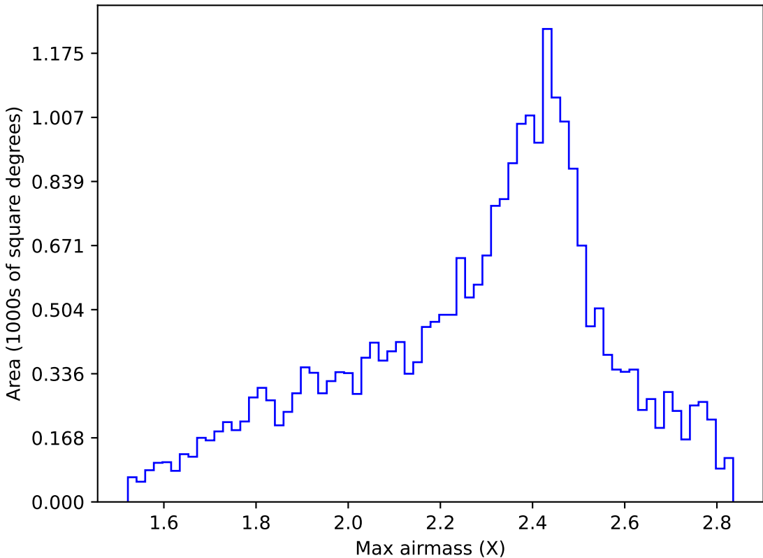
ddf_acor_sf15_lsf30_lsr10_v3.4_10yrs All sky r band: Max airmass
