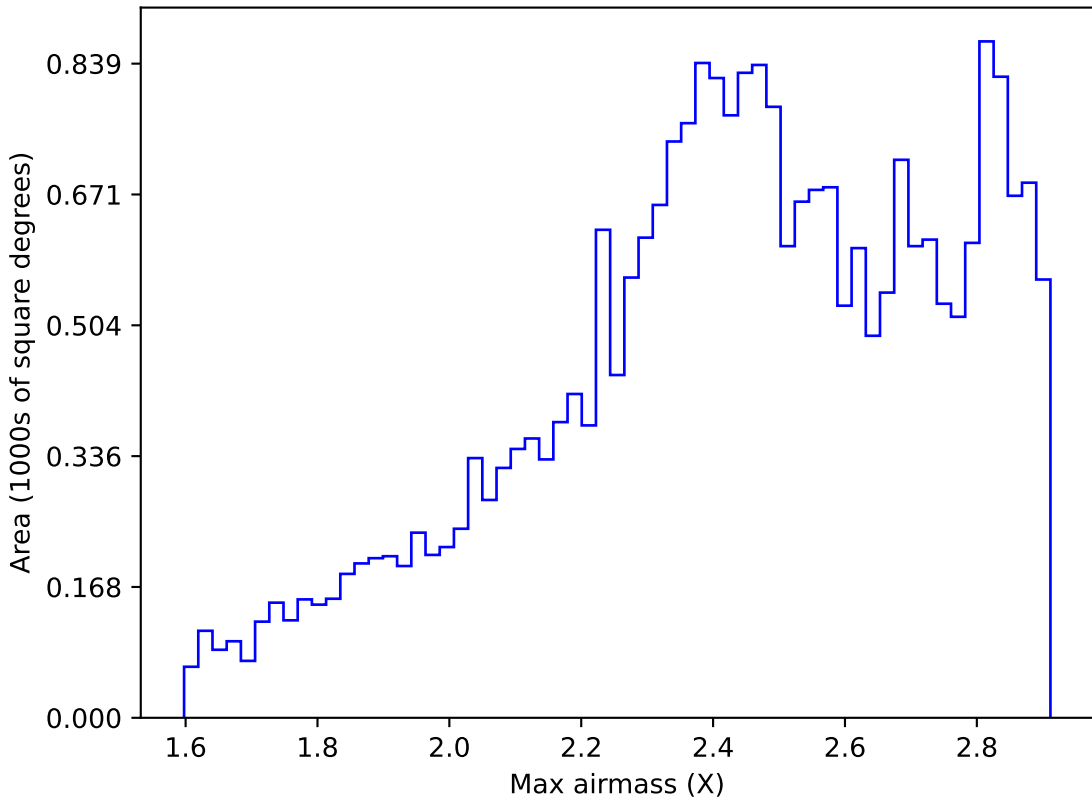
ddf_acor_sf15_lsf30_lsr10_v3.4_10yrs All sky i band: Max airmass
