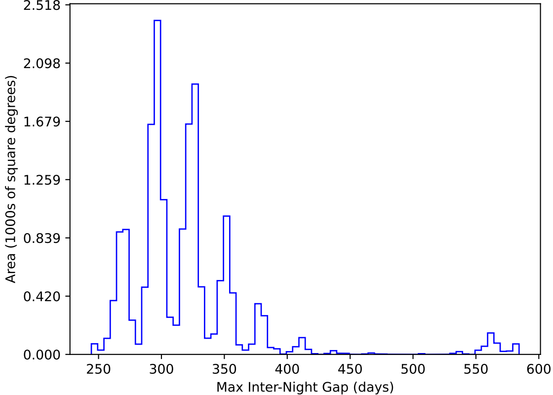
ddf_acor_sf15_lsf30_lsr10_v3.4_10yrs WFD y band: Max Inter-Night Gap
