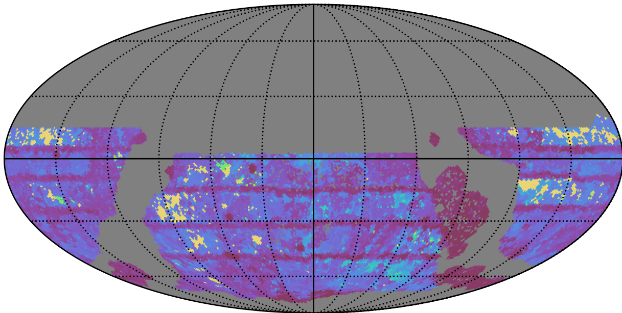
ddf_acor_sf15_lsf30_lsr10_v3.4_10yrs WFD r band: Max Inter-Night Gap
