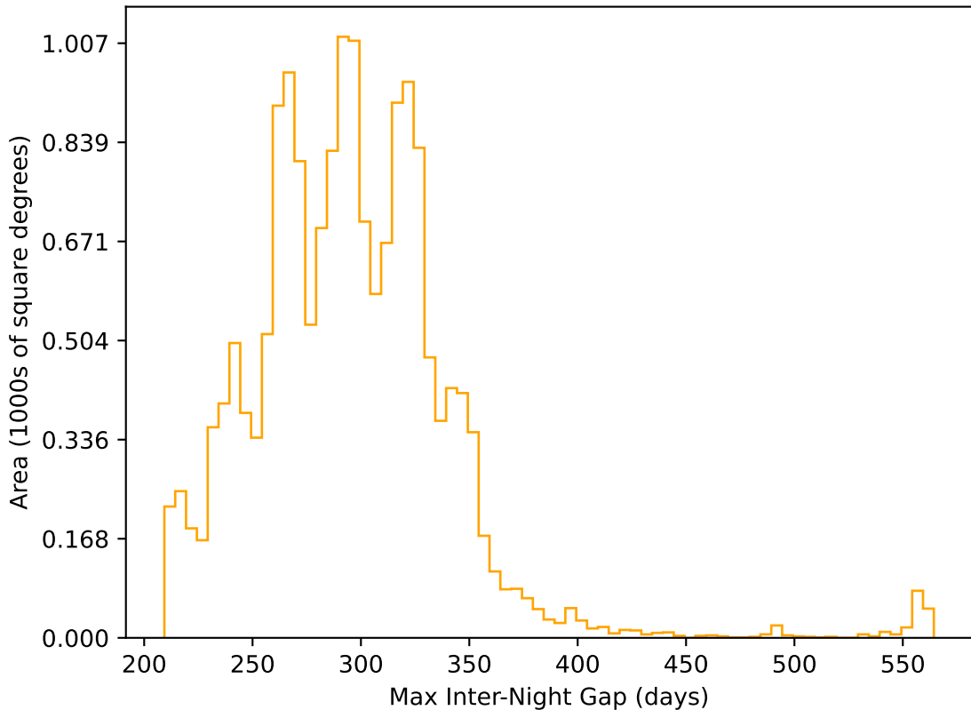
ddf_acor_sf15_lsf30_lsr10_v3.4_10yrs WFD r band: Max Inter-Night Gap
