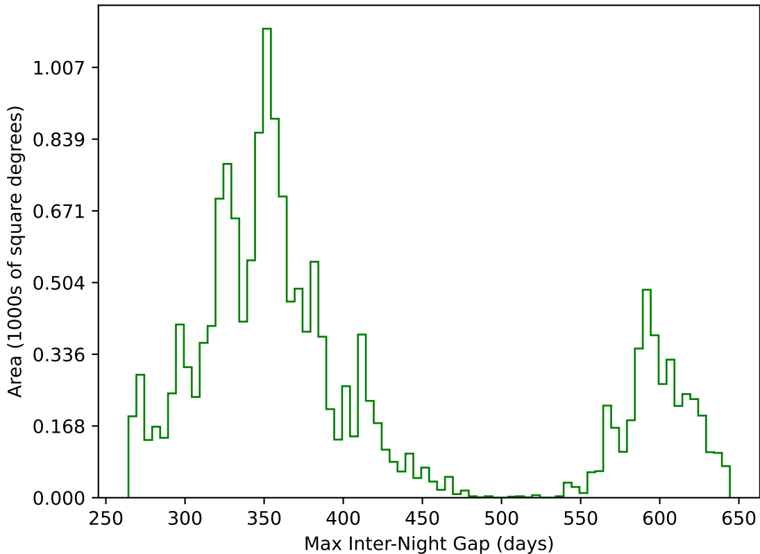
ddf_acor_sf15_lsf30_lsr10_v3.4_10yrs WFD g band: Max Inter-Night Gap
