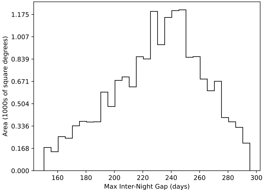
ddf_acor_sf15_lsf30_lsr10_v3.4_10yrs WFD all bands: Max Inter-Night Gap
