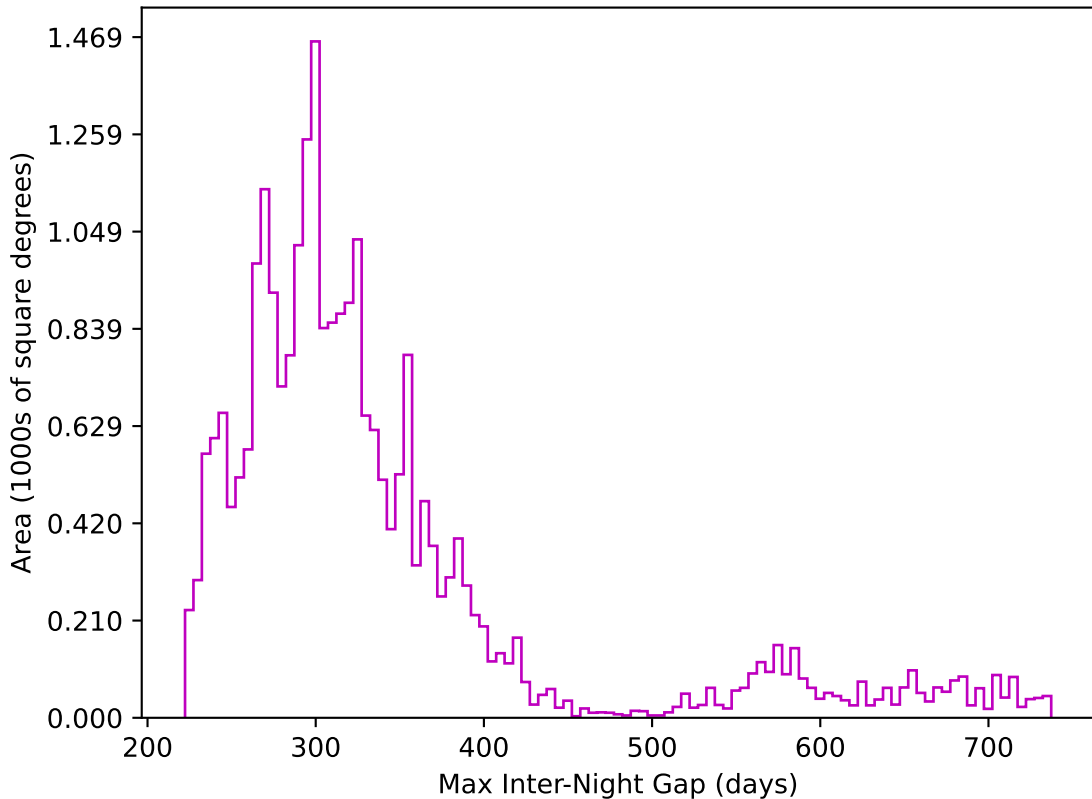
ddf_acor_sf15_lsf30_lsr10_v3.4_10yrs All sky z band: Max Inter-Night Gap
