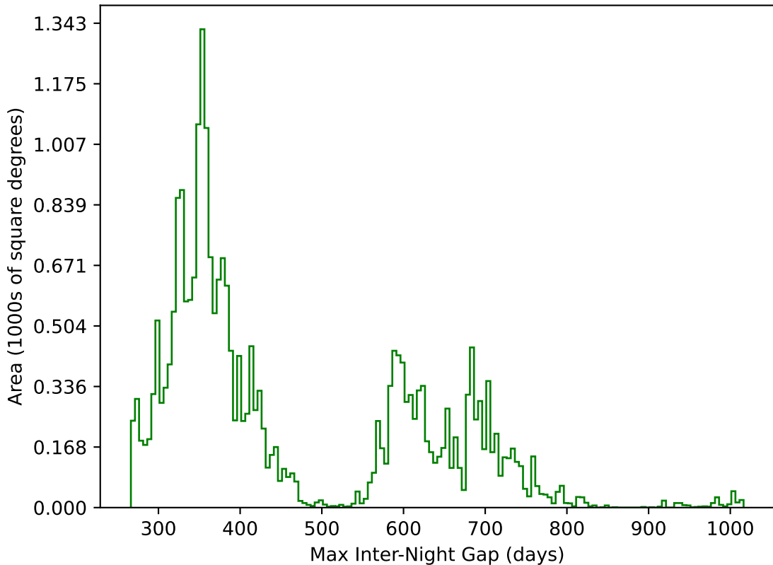
ddf_acor_sf15_lsf30_lsr10_v3.4_10yrs All sky g band: Max Inter-Night Gap
