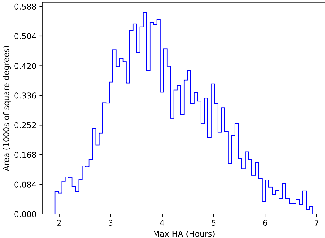
ddf_acor_sf15_lsf30_lsr10_v3.4_10yrs WFD u band: Max HA
