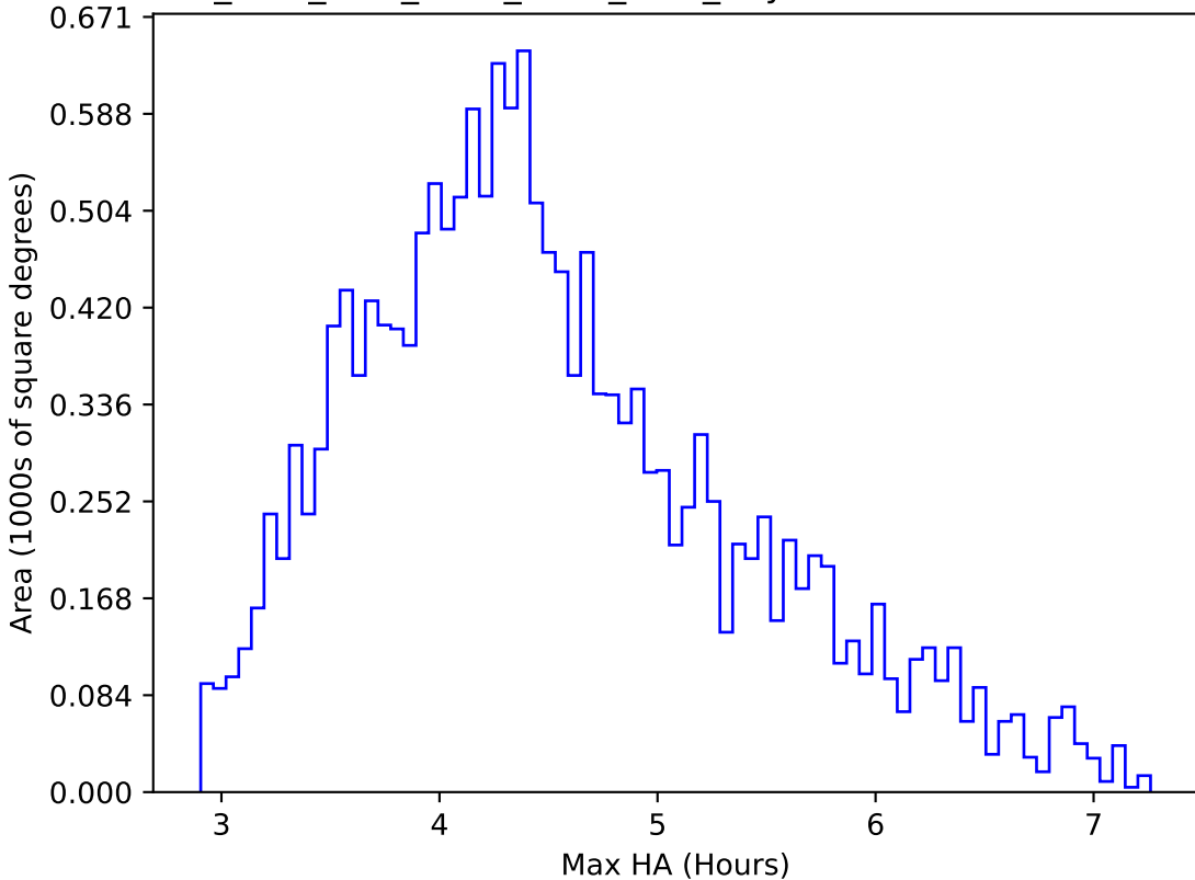
ddf_acor_sf15_lsf30_lsr10_v3.4_10yrs WFD r band: Max HA
