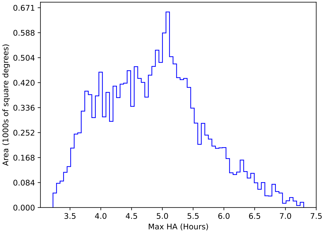
ddf_acor_sf15_lsf30_lsr10_v3.4_10yrs WFD i band: Max HA
