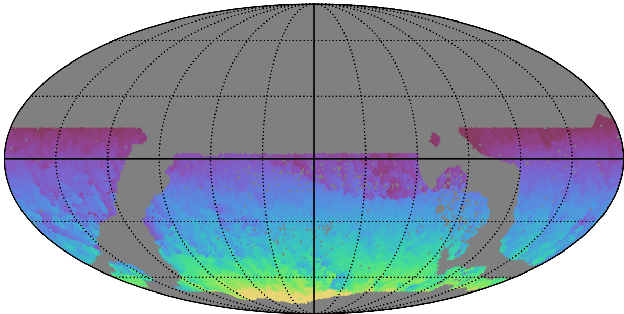
ddf_acor_sf15_lsf30_lsr10_v3.4_10yrs WFD all bands: Max HA
