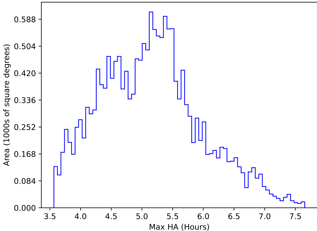
ddf_acor_sf15_lsf30_lsr10_v3.4_10yrs WFD all bands: Max HA
