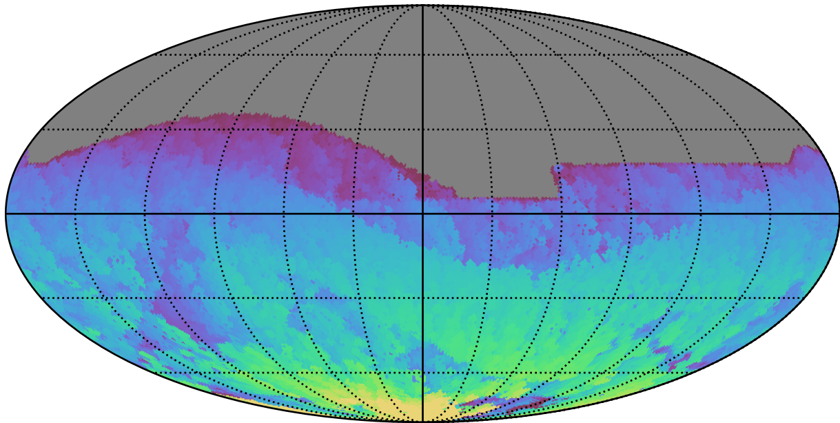
ddf_acor_sf15_lsf30_lsr10_v3.4_10yrs All sky z band: Max HA
