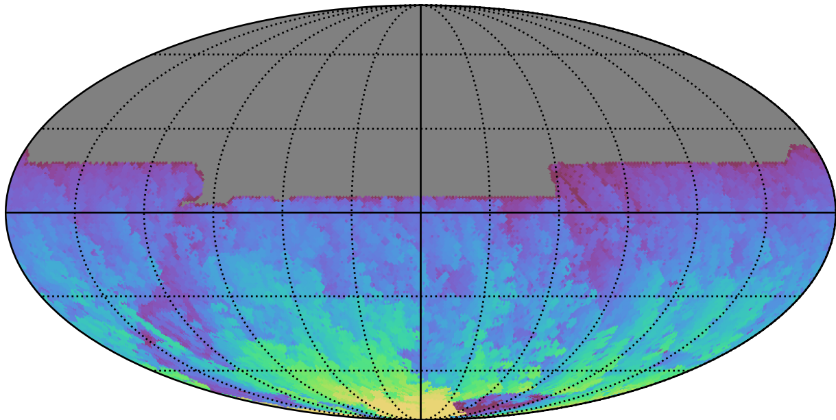
ddf_acor_sf15_lsf30_lsr10_v3.4_10yrs All sky y band: Max HA
