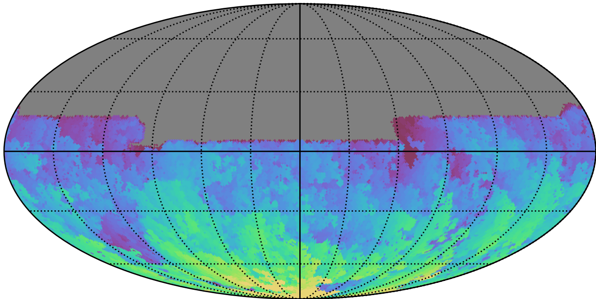
ddf_acor_sf15_lsf30_lsr10_v3.4_10yrs All sky u band: Max HA
