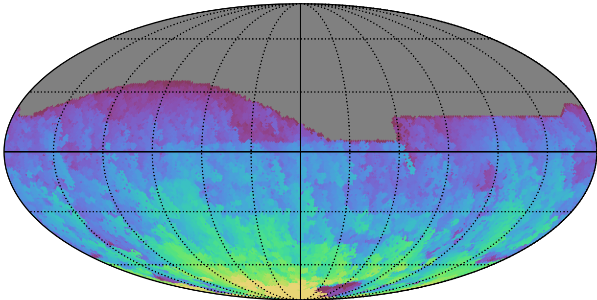
ddf_acor_sf15_lsf30_lsr10_v3.4_10yrs All sky r band: Max HA
