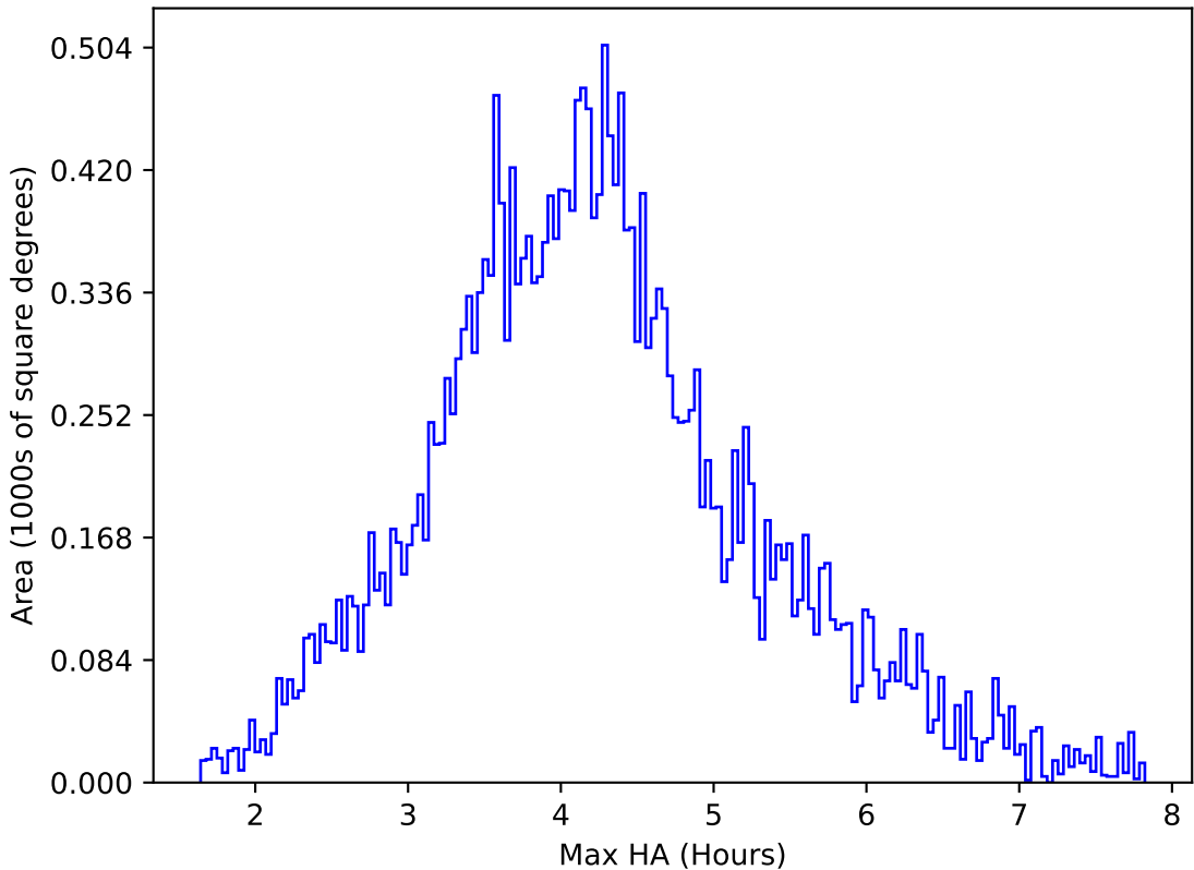
ddf_acor_sf15_ls30_lsr10_v3.4_10yrs All sky r band: Max HA
