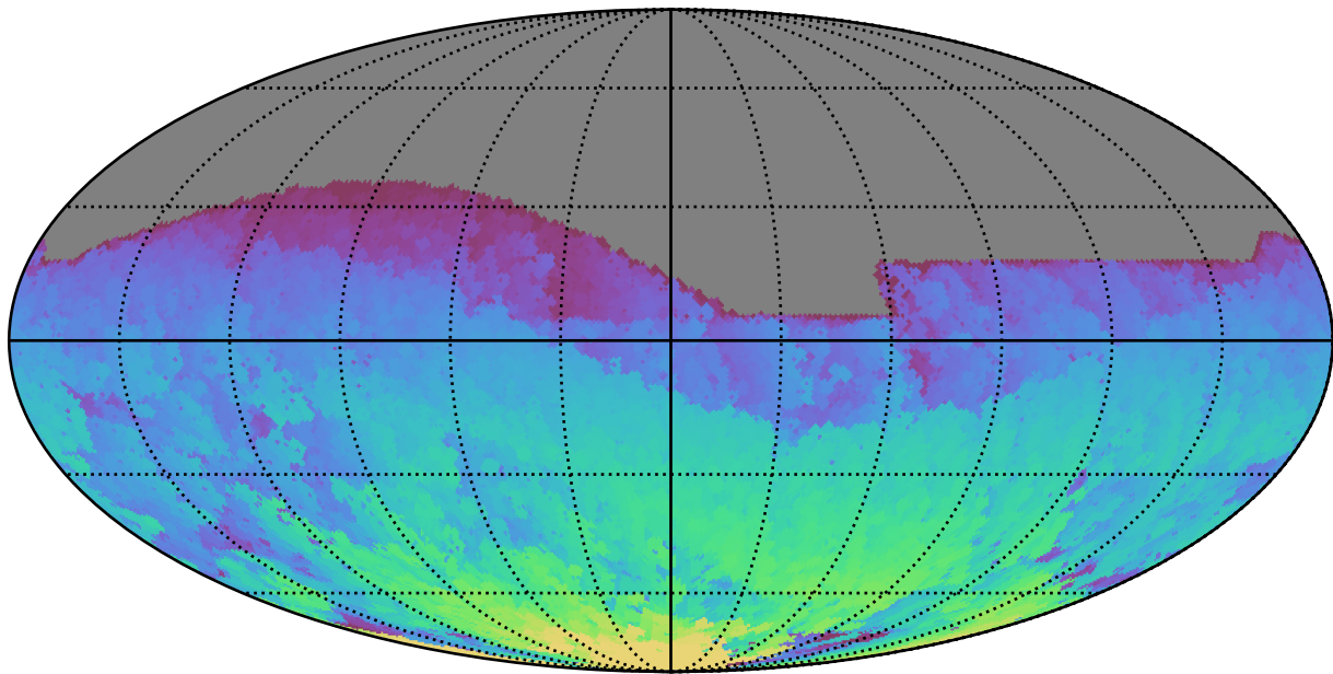
ddf_acor_sf15_lsf30_lsr10_v3.4_10yrs All sky i band: Max HA
