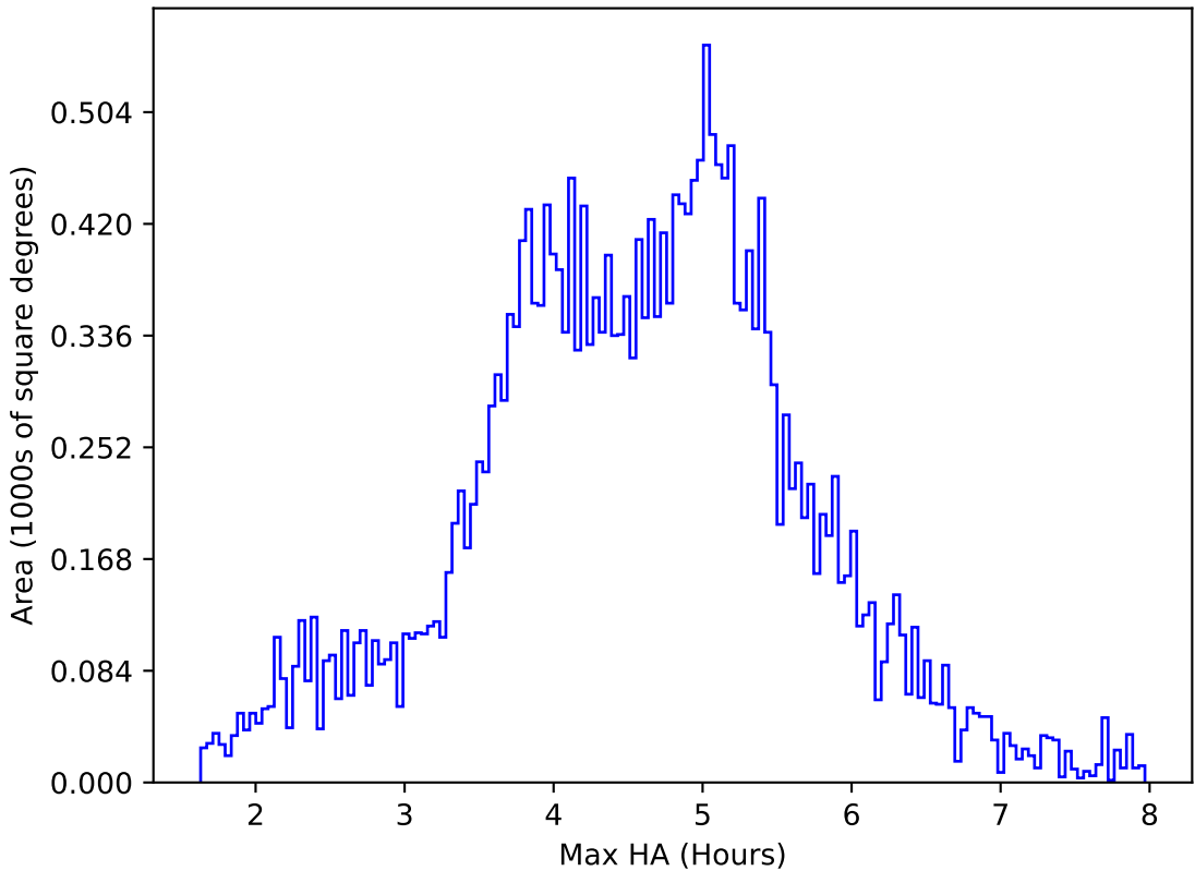
ddf_acor_sf15_lsf30_lsr10_v3.4_10yrs All sky i band: Max HA
