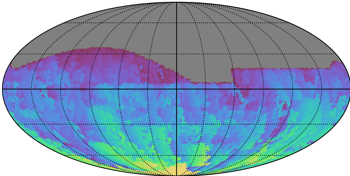
ddf_acor_sf15_lsf30_lsr10_v3.4_10yrs All sky g band: Max HA
